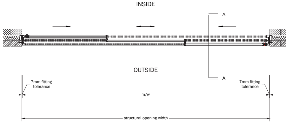
PROPOSED FRAME LAYOUTS & PROJECTED EXTERNAL ELEVATION Scale 1:25 @ A3
