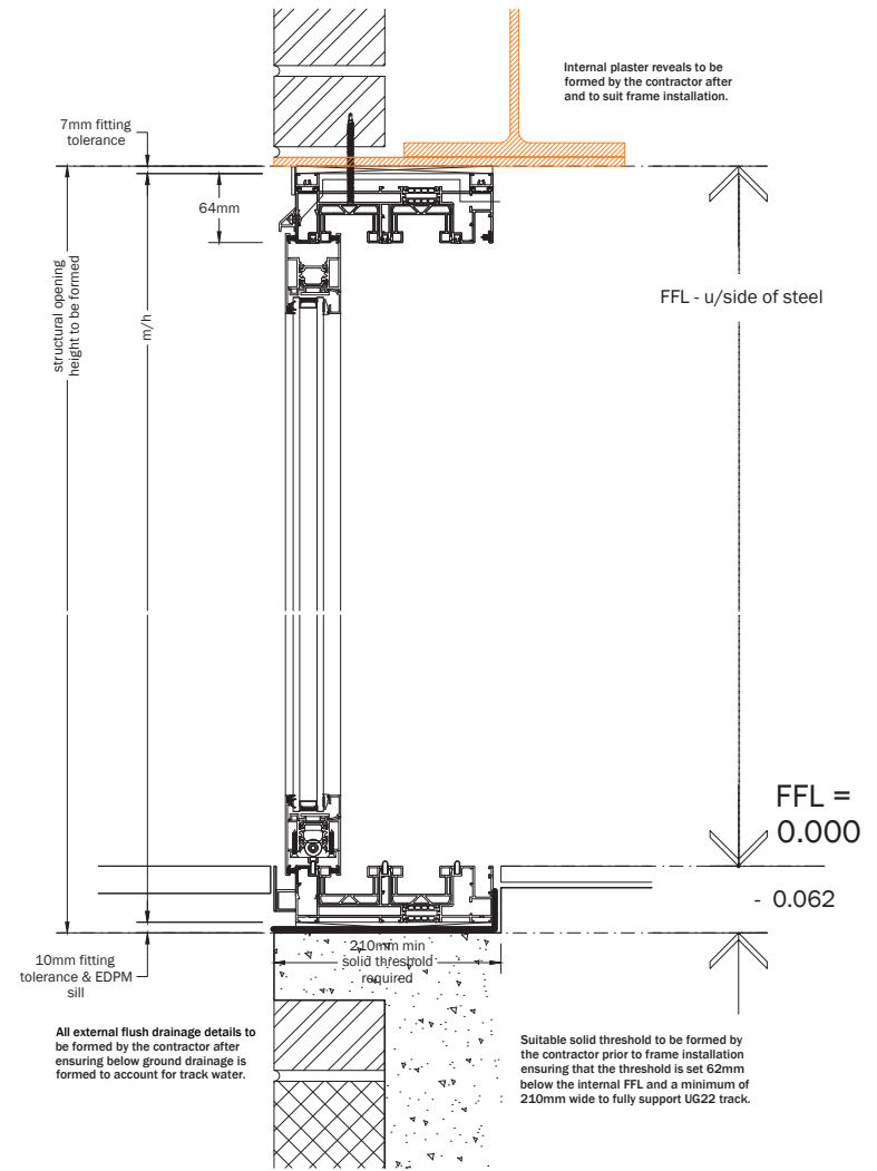
Height Section A-A
