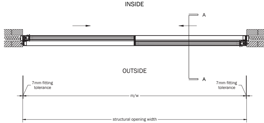
PROPOSED FRAME LAYOUTS & PROJECTED EXTERNAL ELEVATION Scale 1:25 @ A3
